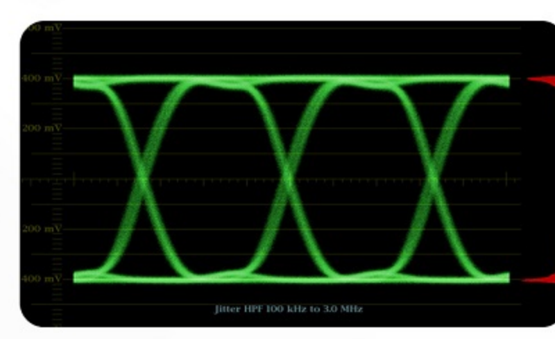
Eye Diagram
